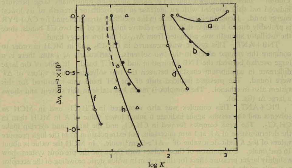
FIG. 5.—Relation between \Delta\nu and \log K ; lettering of curves as in fig. 3.
